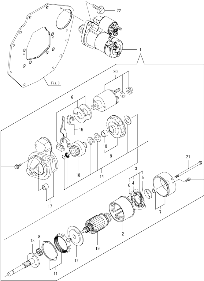
Fig.14. STARTING MOTOR
