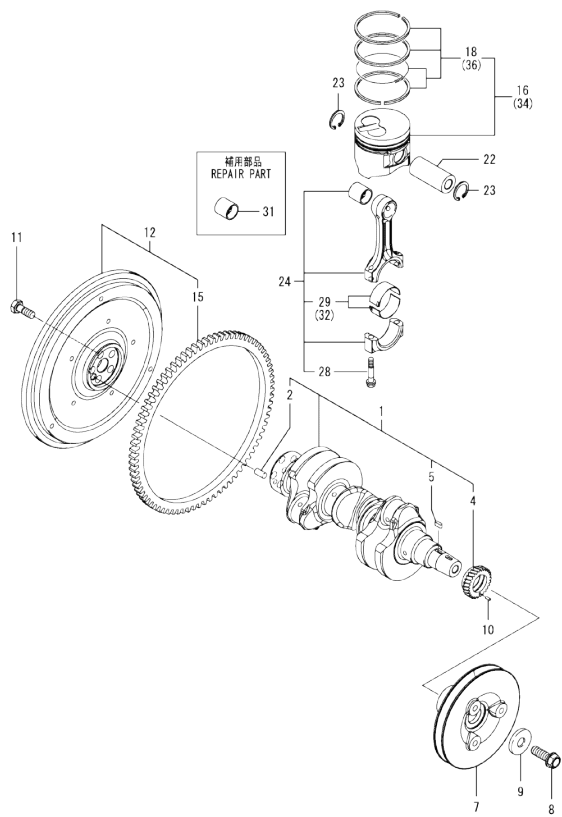
Fig.7. CRANKSHAFT & PISTON
